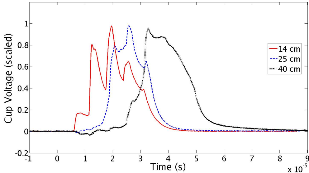
Figure 4.9 Moving the cup away from the source shows a delay in the signal. The amplitude decreases significantly with separation, so all signals are scaled to a range of -1 to 1. The 14 cm signal is scaled down by a factor of roughly 16.9, the 25 cm by a factor of 5.6, and the 40 cm by a factor of 1.6.
