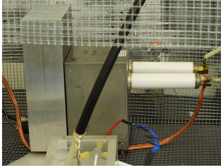
Figure 3.2 The pulse transformer.
