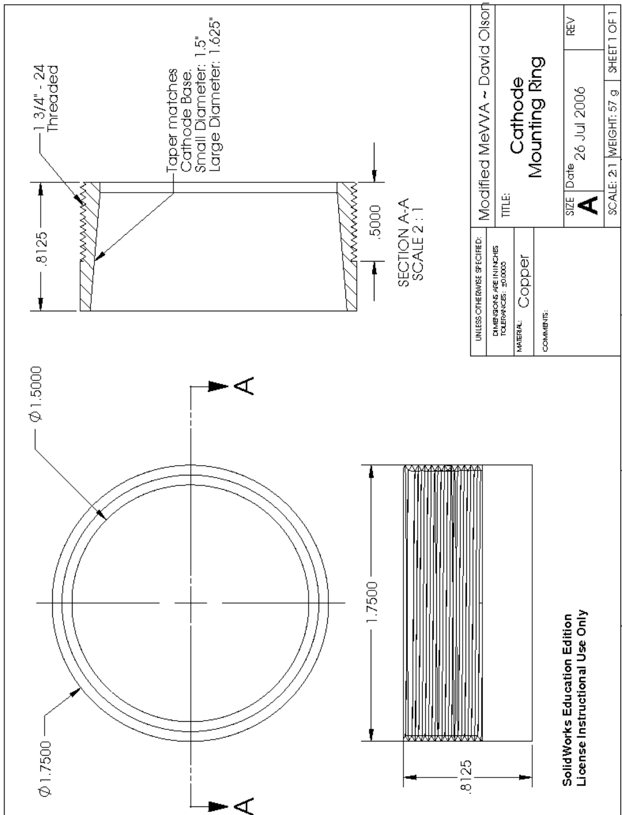
Figure A.6 Cathode Mounting Ring Machining Drawing
